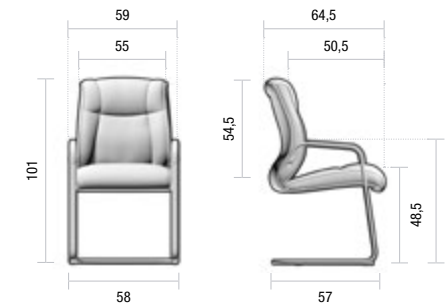
Confidente Confident / Luge / Cantilever / Freischwinger.
